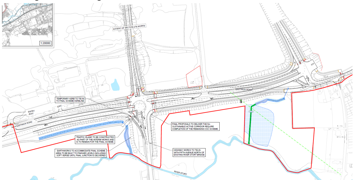
Figure 21: Extract of Central Stort Crossing Interim Junction Tie-In General Arrangement Drawing VD17516-CCi-100-GA REV P03
