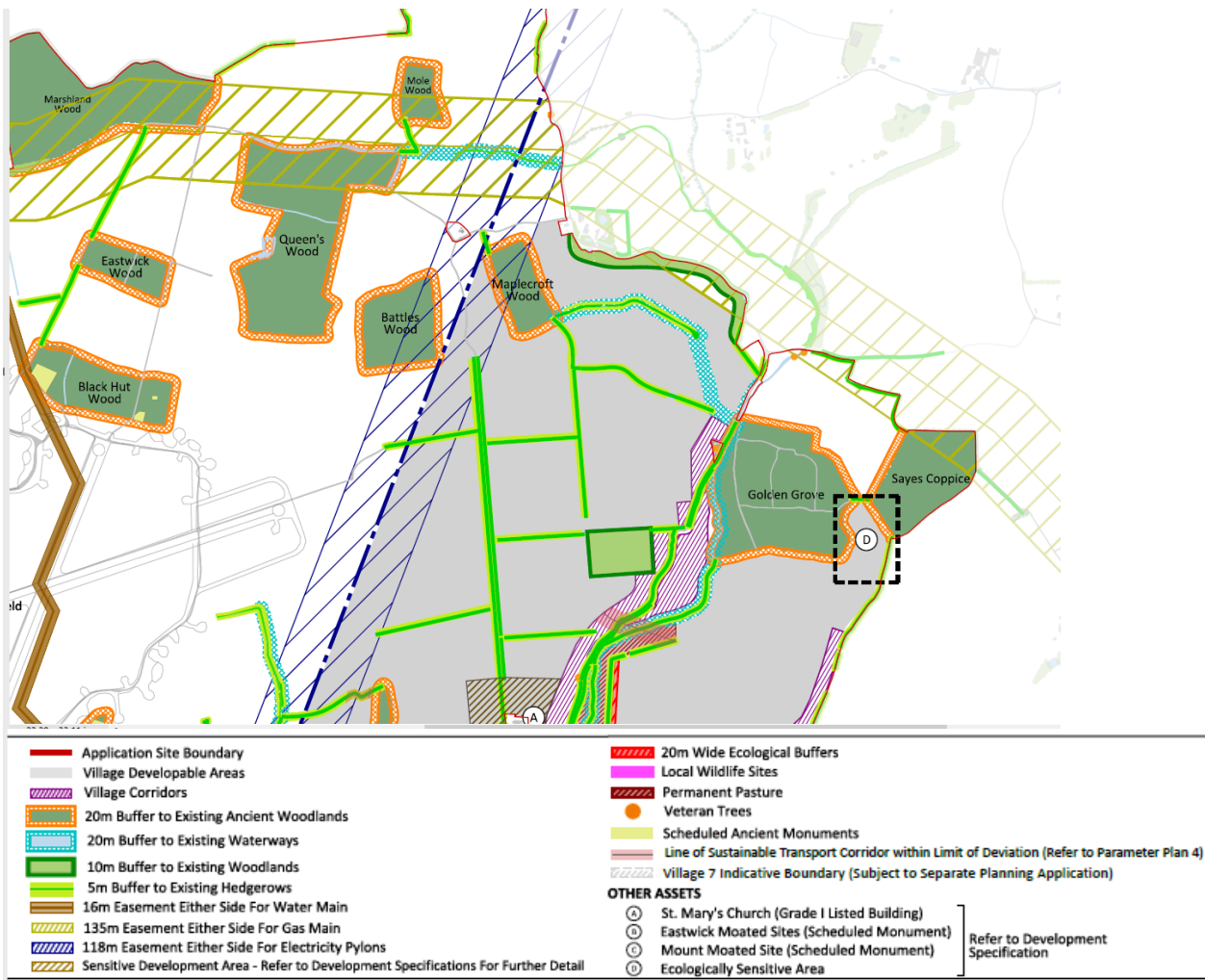
Figure 18 Extract parameter Plan 2 – Golden Grove /Sayes Coppice
